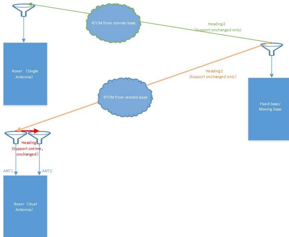
Figure 3-1 Heading Schematic
